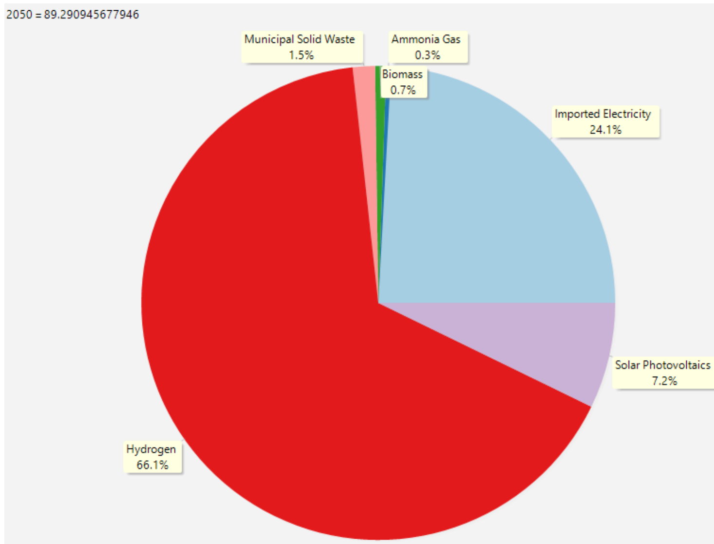
Figure 9: Percentage share of electricity generation by feedstock fuel type in 2050 (HA1)
